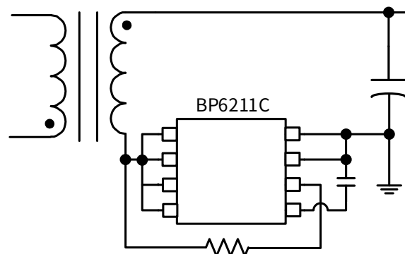
Figure 1. BP6211C Typical Application
