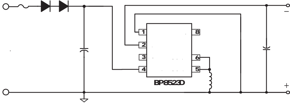
Figure 2. Typical buck-boost application with the BP8523D
